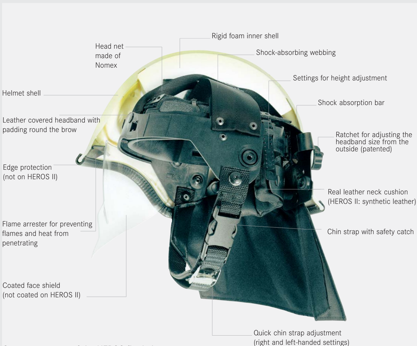
Component parts of the HEROS fire helmet
